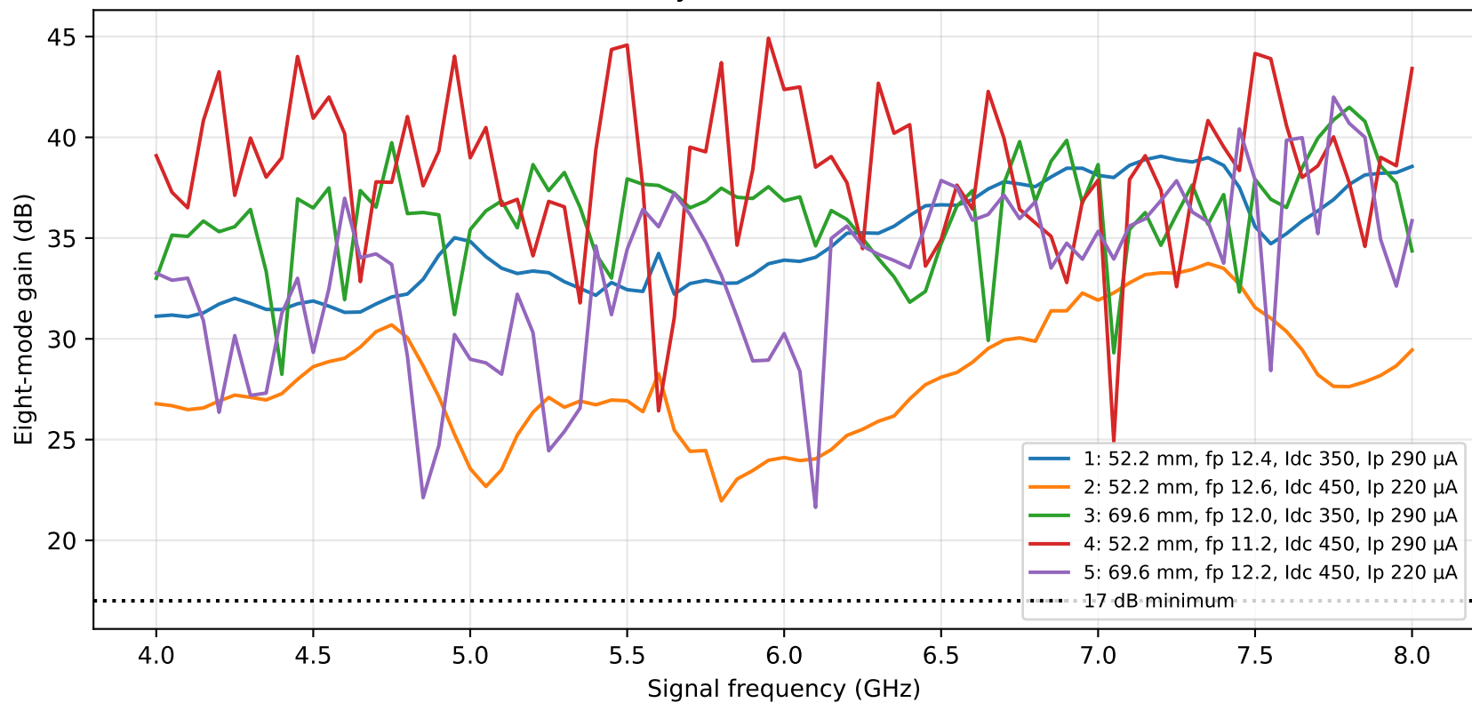
13-3-13: densely verified nonlinear candidates
