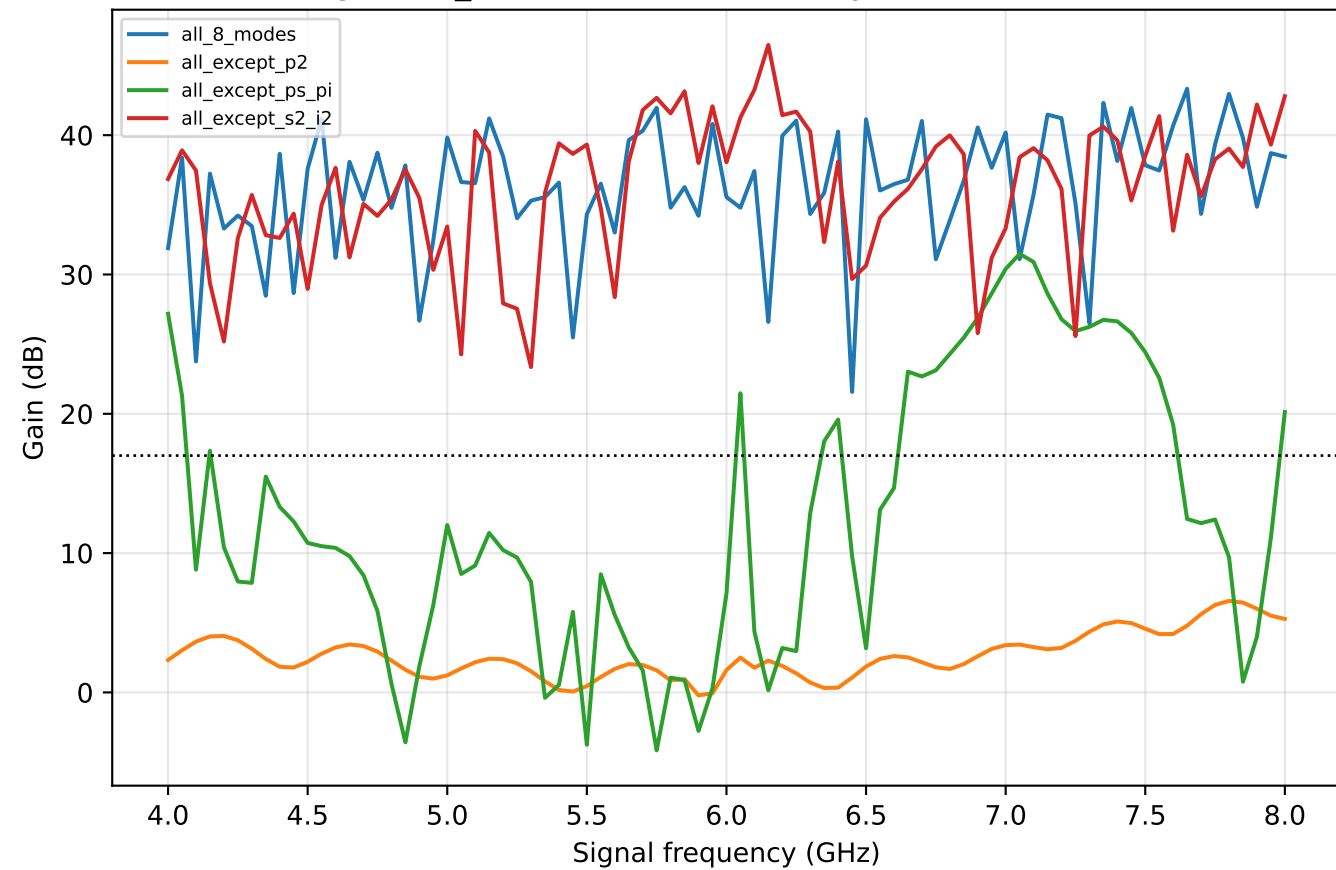
general_ideal: remove one family from all modes
