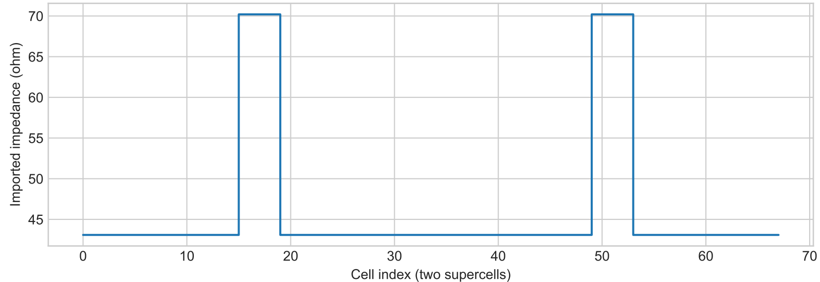
HFSS-selected cell pattern
