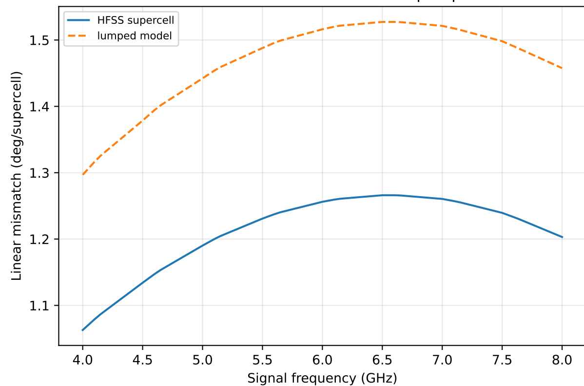
3WM mismatch at 13.13 GHz pump
