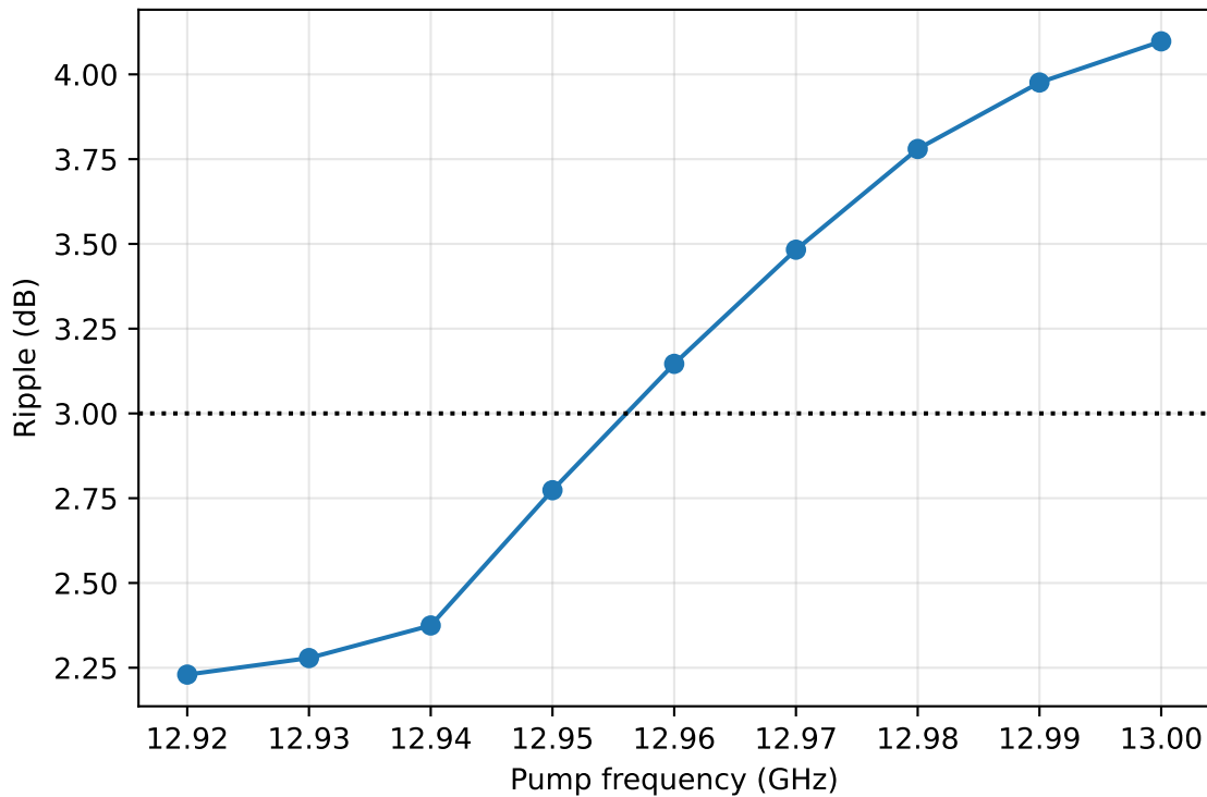
Pump-frequency sensitivity
