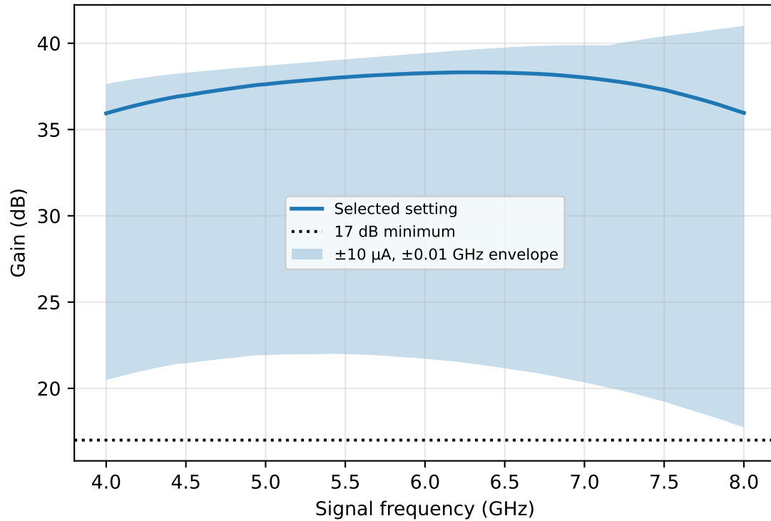
Pump-frequency sensitivity
