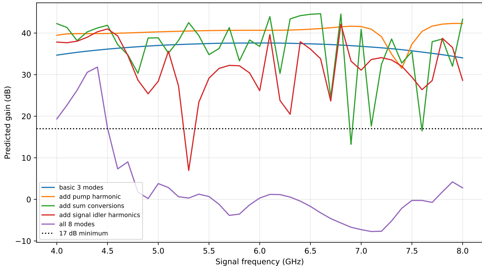
Ideal-model mode ablation at 12.94 GHz
