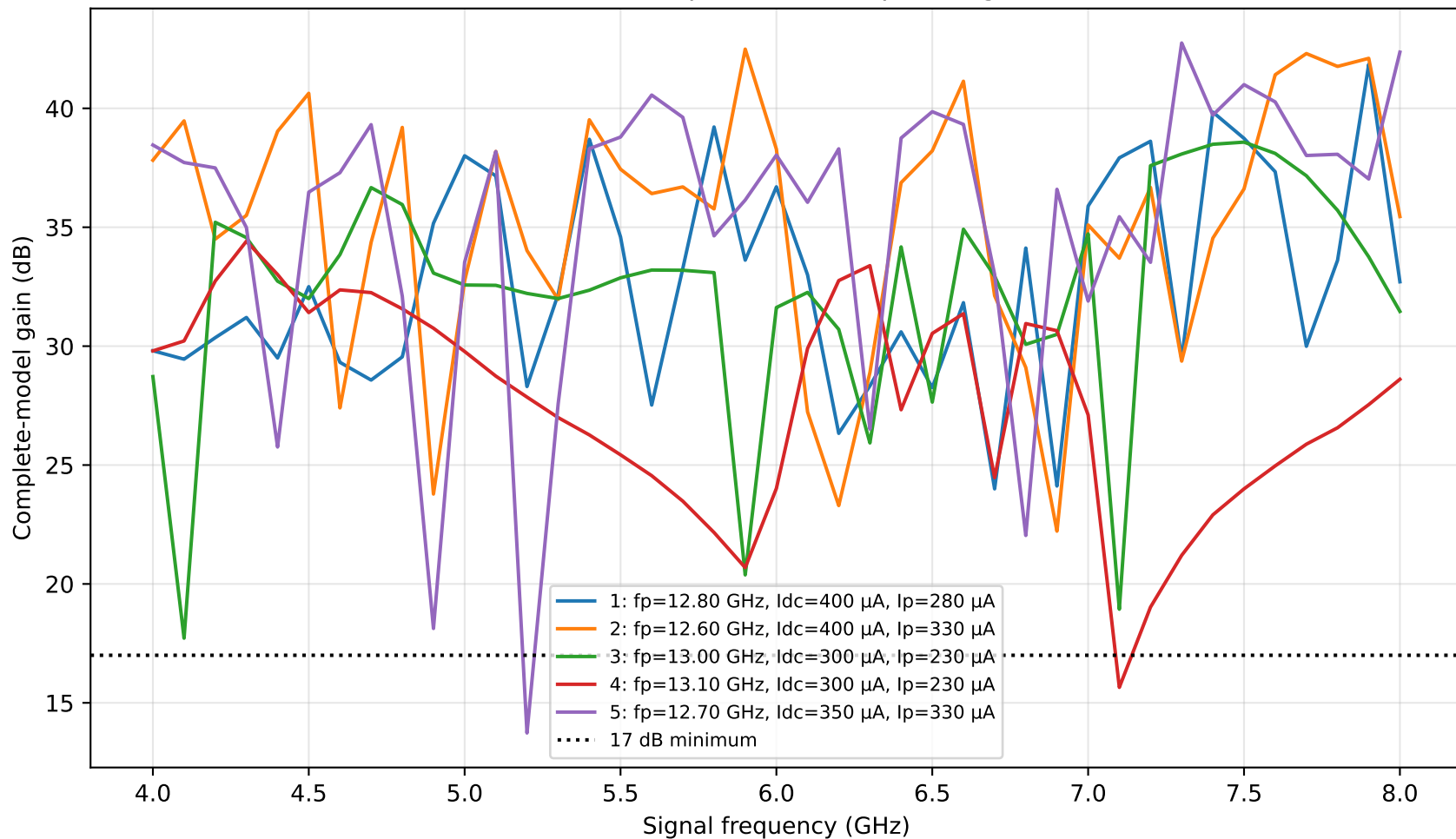
Fine-HFSS complete-model operating scan
