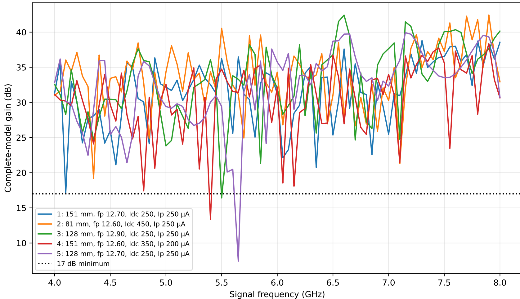
Lower-drive, longer-line candidates
