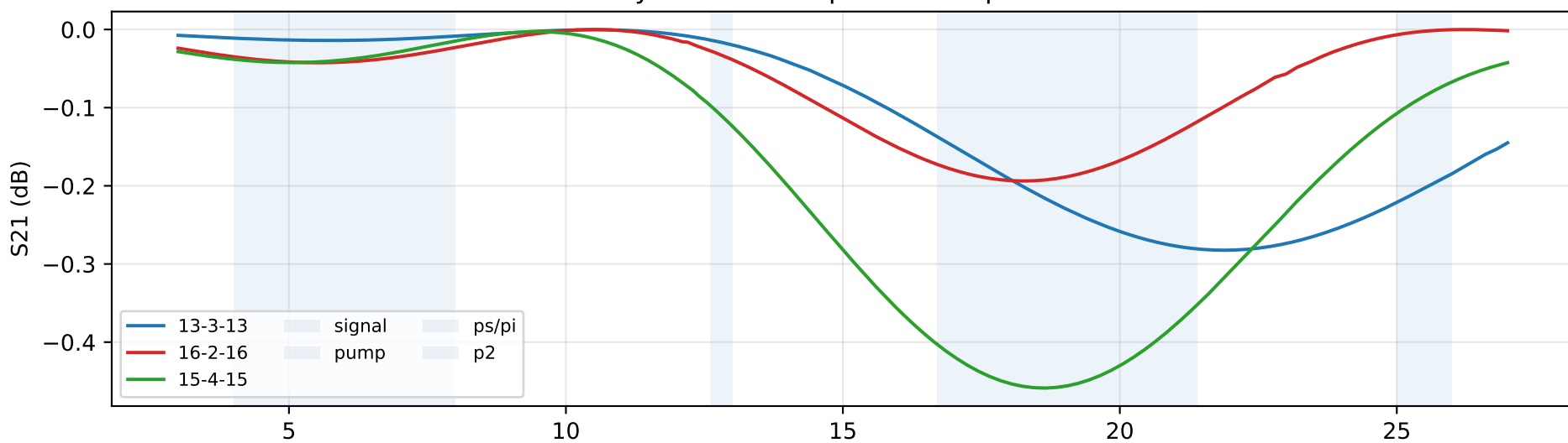
Physical HFSS supercell comparison
