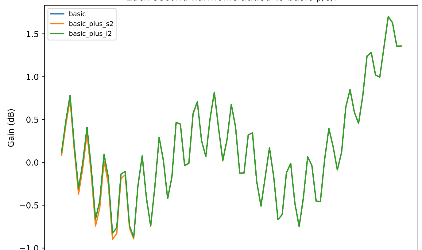
Gain versus harmonic mismatch
