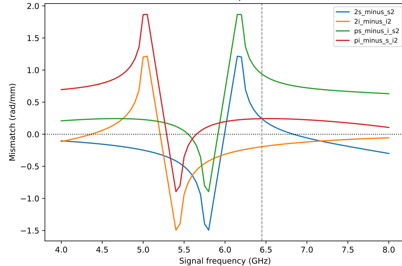
Second-harmonic linear phase mismatches
