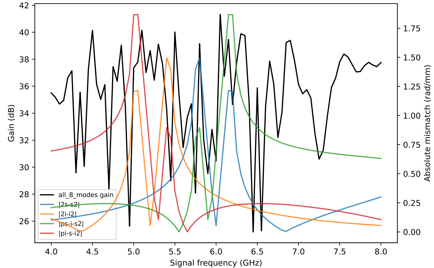
Gain versus harmonic mismatch
