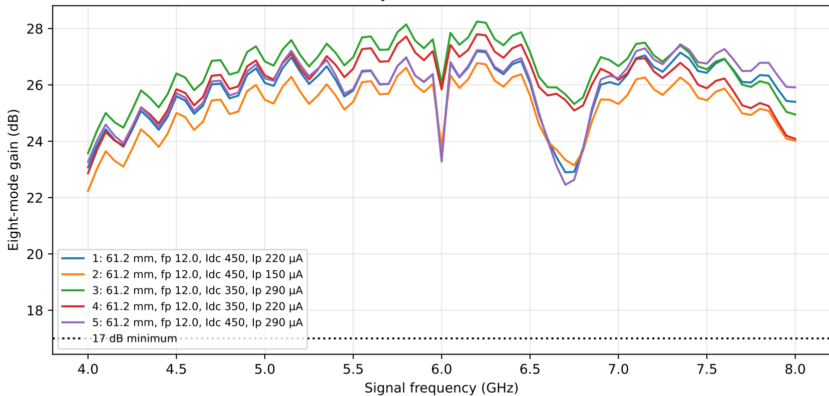
15-4-15: densely verified nonlinear candidates
