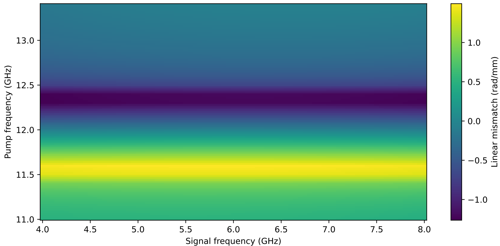
15-4-15: densely verified nonlinear candidates
