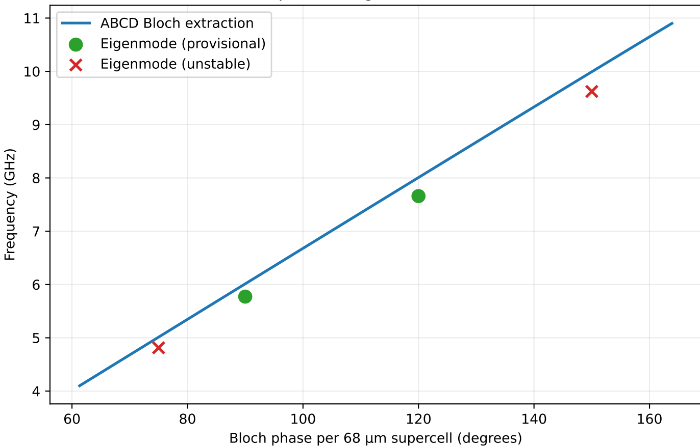
16-2-16 periodic eigenmode cross-check
