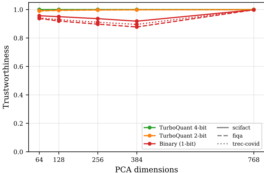
Trustworthiness vs. Dimension (k=10)
