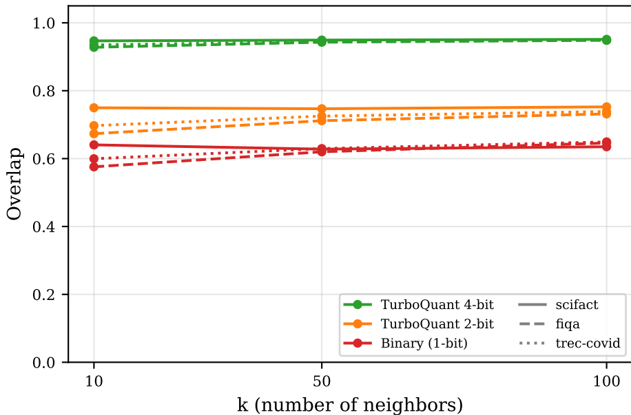
Overlap (d=768)
