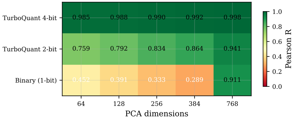
scifact — Pearson r
