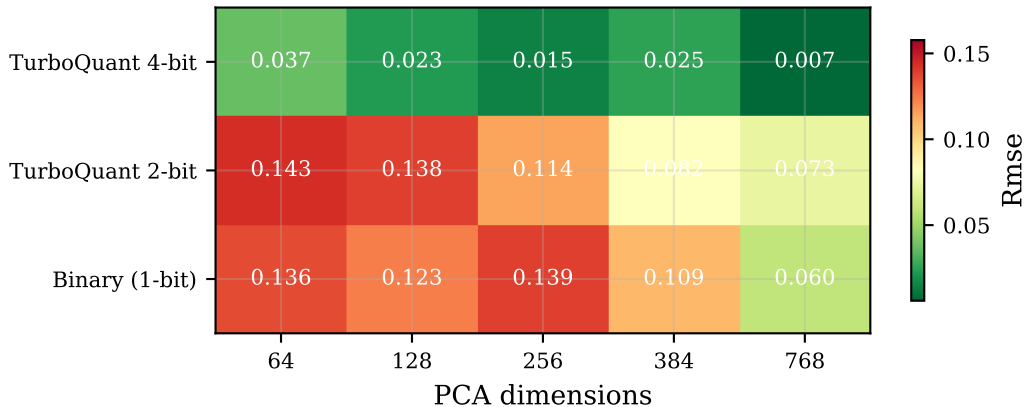
scifact — RMSE
