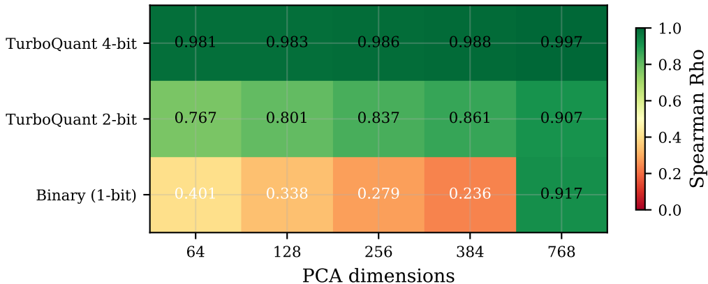
trec-covid — Spearman \rho
