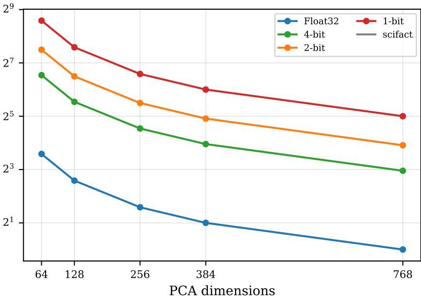
Compression vs. 768d Float32
