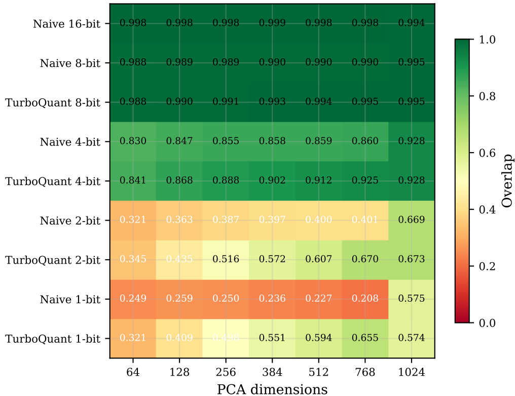
fiqa — Overlap (k=10)
