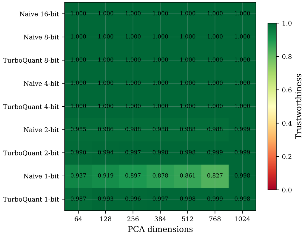
fiqa — Trustworthiness (k=10)
