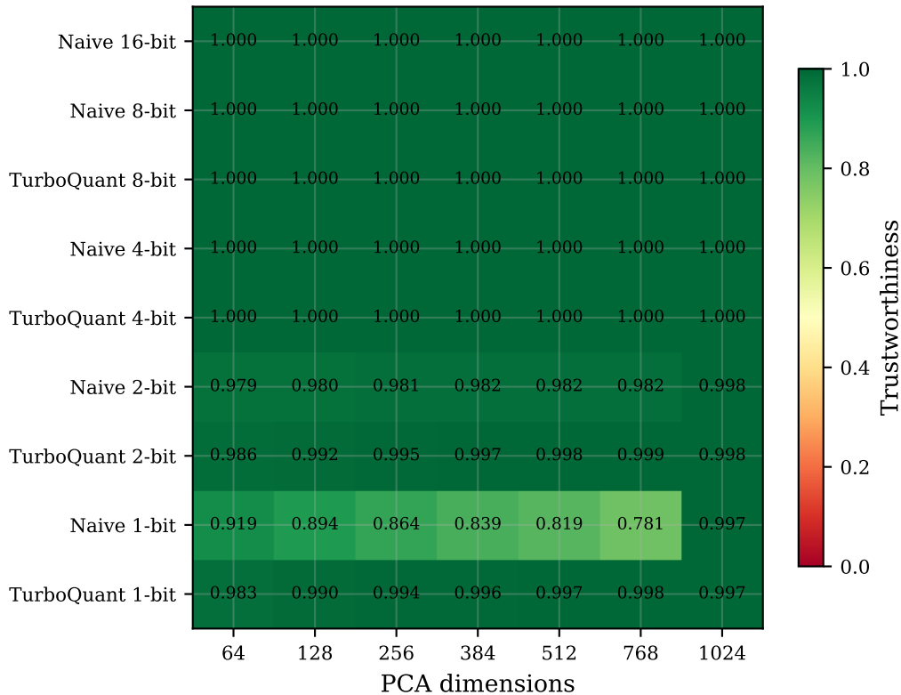
fiqa — Trustworthiness (k=20)
