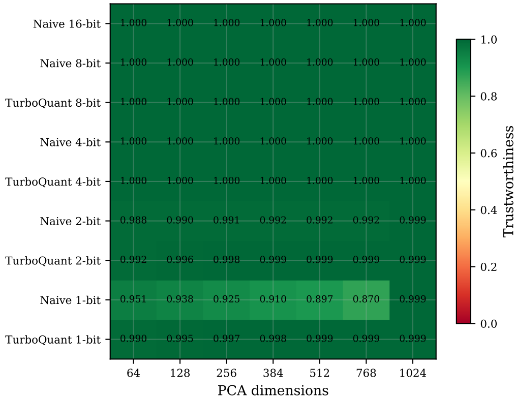
fiqa — Trustworthiness (k=5)
