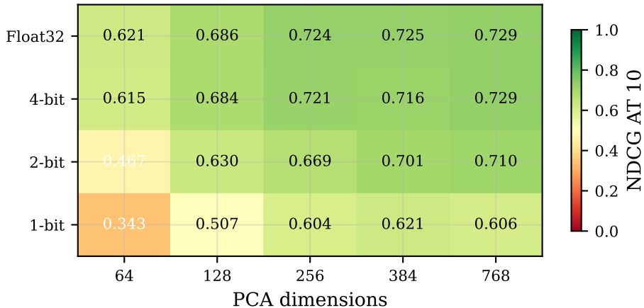
scifact - NDCG@10
