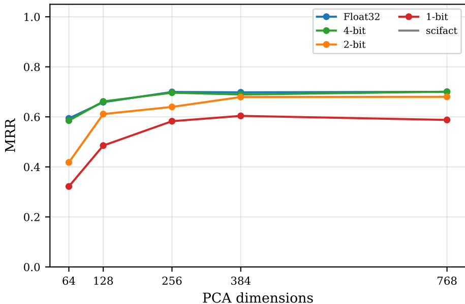
Retrieval MRR by Dimension
