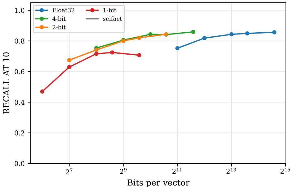
Retrieval RECALL AT 10 vs. Compression
