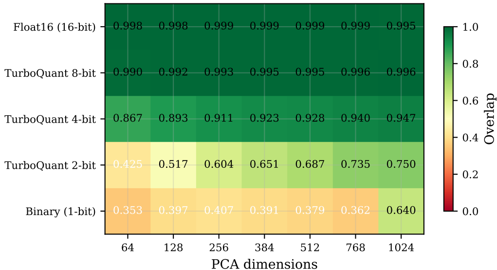
scifact — Overlap (k=10)
