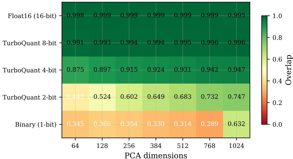
scifact — Overlap (k=20)
