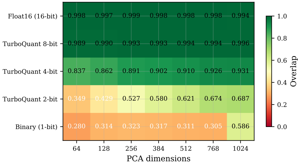
trec-covid — Overlap (k=5)
