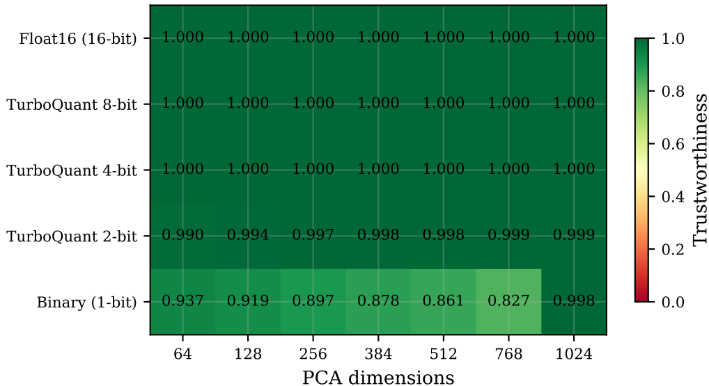
fiqa — Trustworthiness (k=10)
