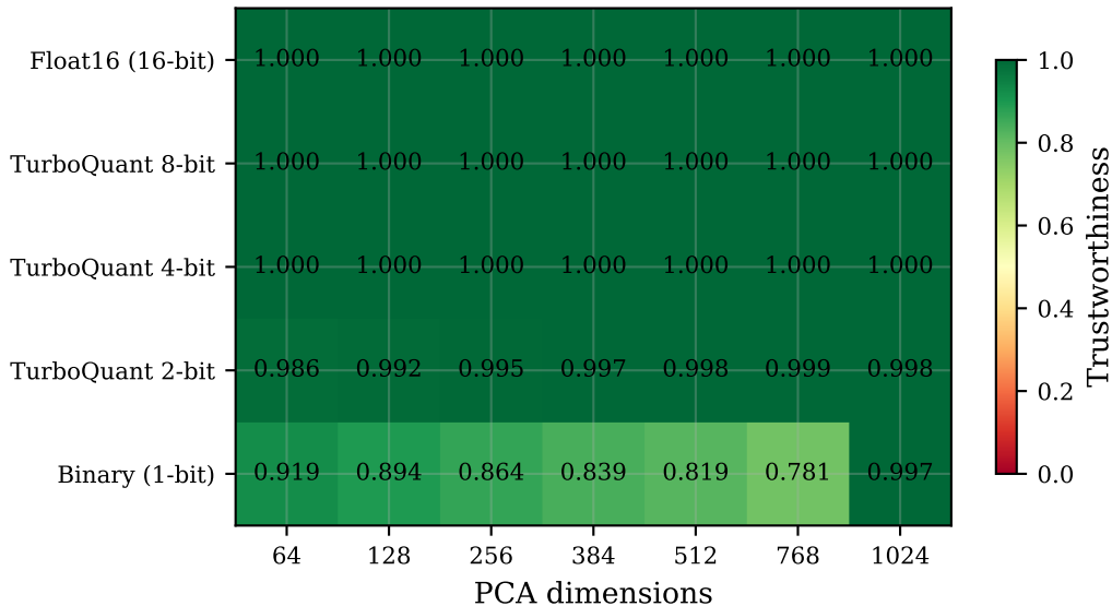
fiqa — Trustworthiness (k=20)
