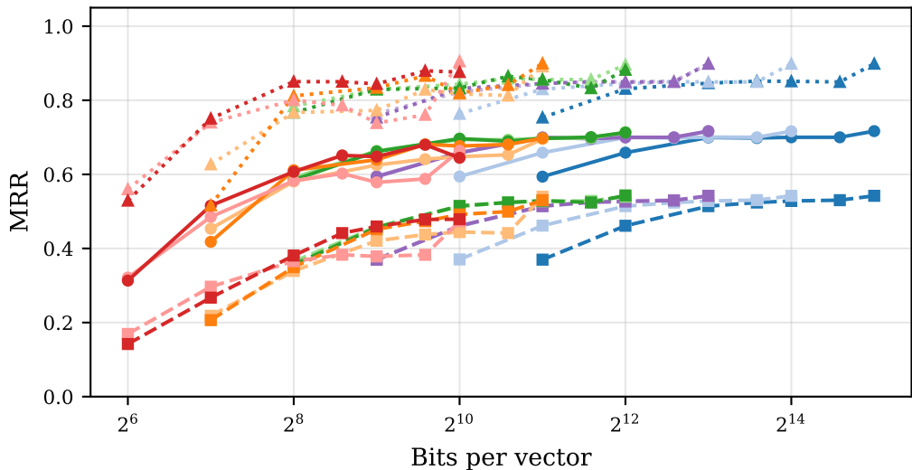
Retrieval MRR vs. Compression
