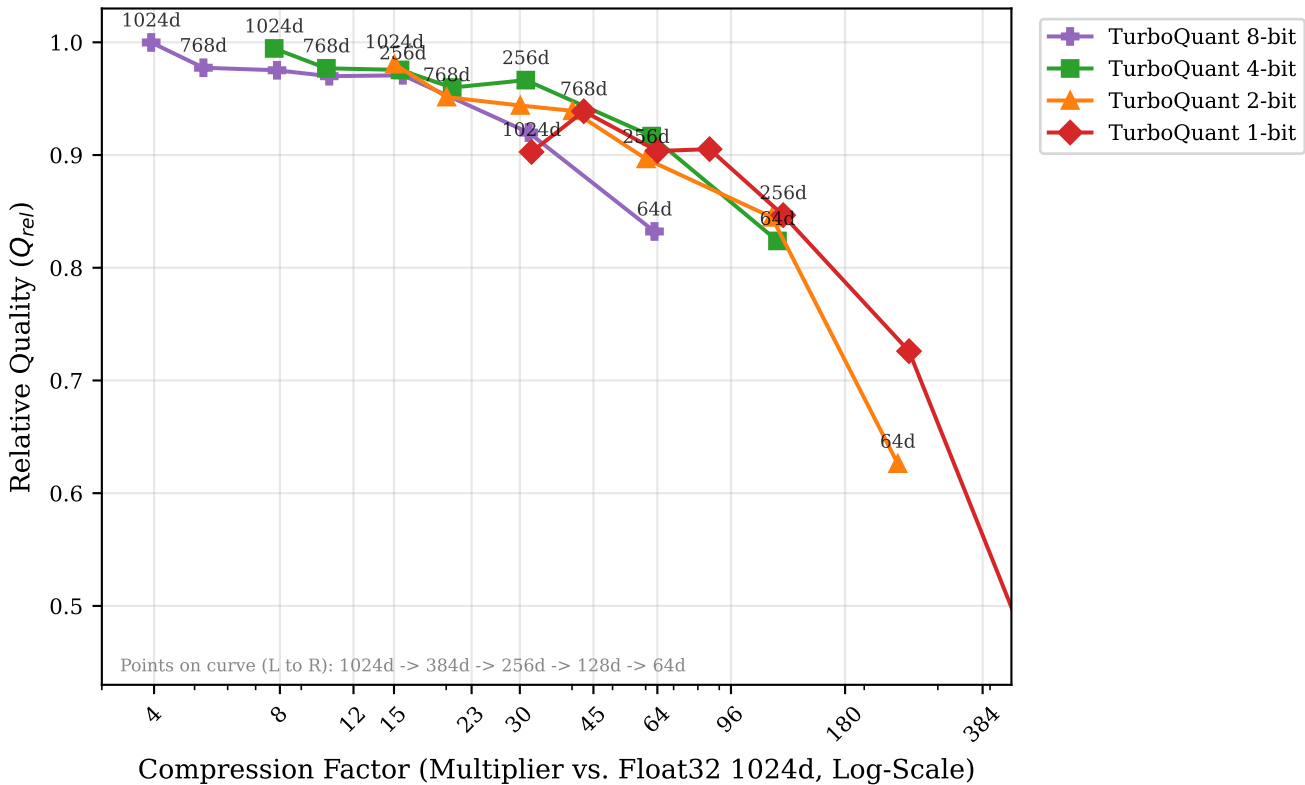
Quality vs. Compression Factor (TurboQuant Only)
