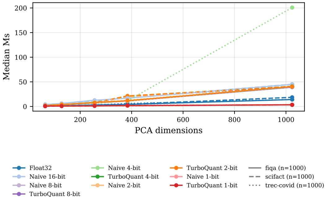
NumPy pairwise distance
