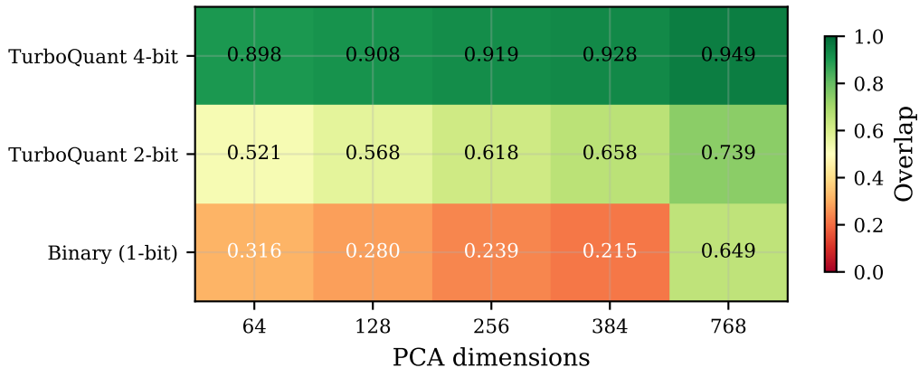
trec-covid — Overlap (k=100)
