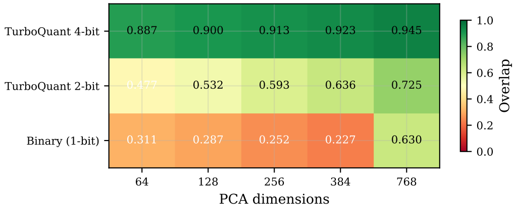
trec-covid — Overlap (k=50)
