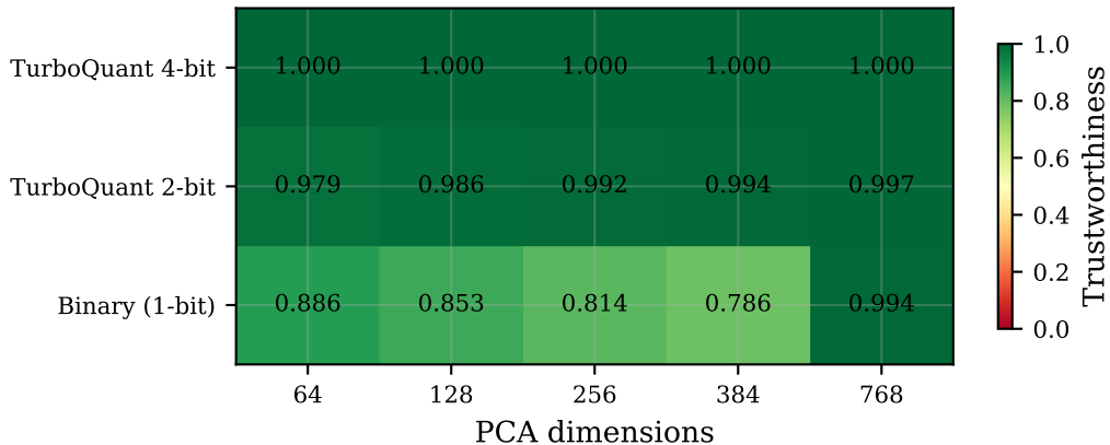
fiqa — Trustworthiness (k=50)
