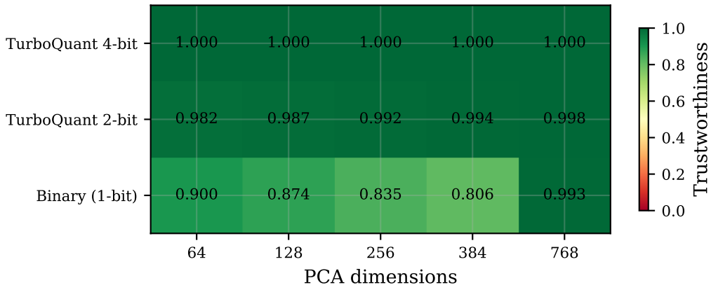
scifact — Trustworthiness (k=50)
