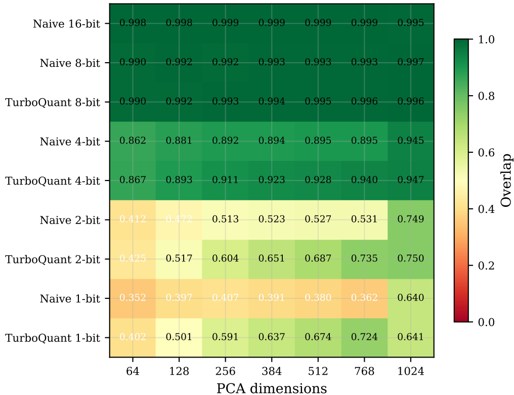
scifact — Overlap (k=10)
