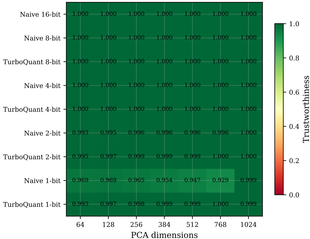
scifact — Trustworthiness (k=5)
