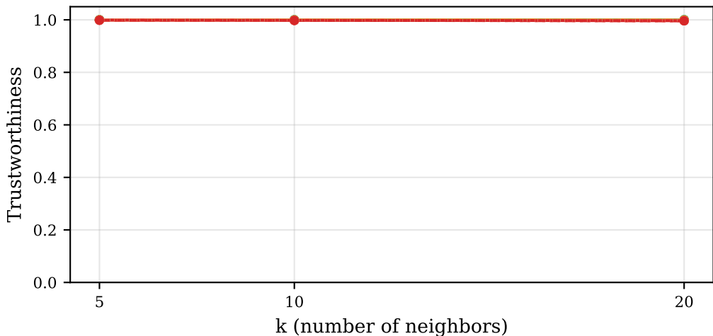
Trustworthiness (d=1024)
