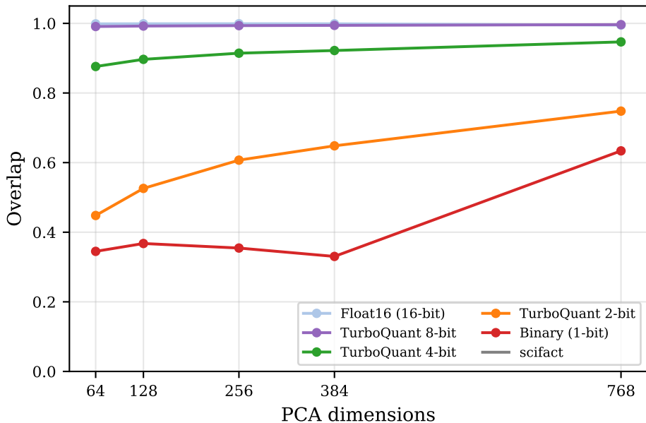
Overlap vs. Dimension (k=20)
