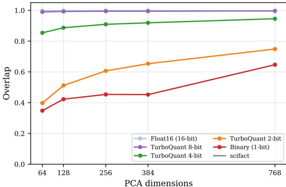
Overlap vs. Dimension (k=5)
