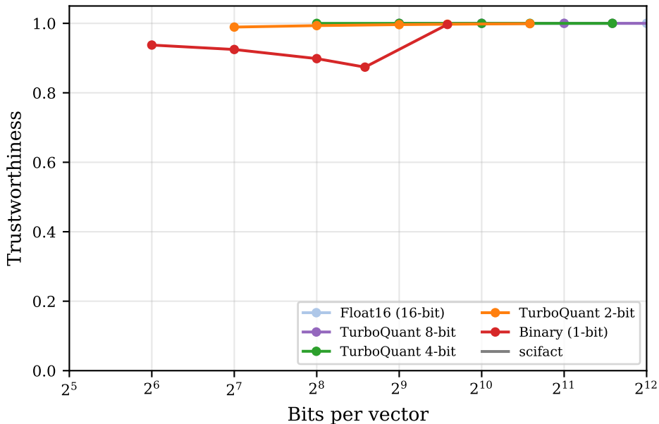
Trustworthiness vs. Compression (k=20)
