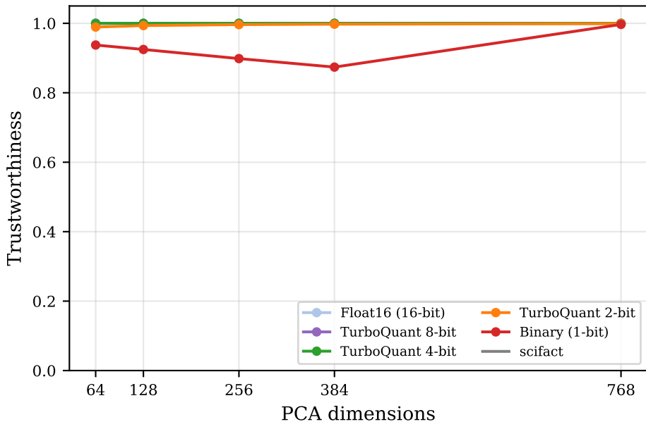
Trustworthiness vs. Dimension (k=20)
