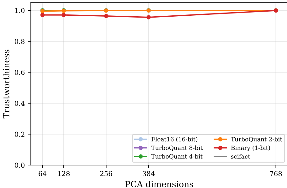
Trustworthiness vs. Dimension (k=5)
