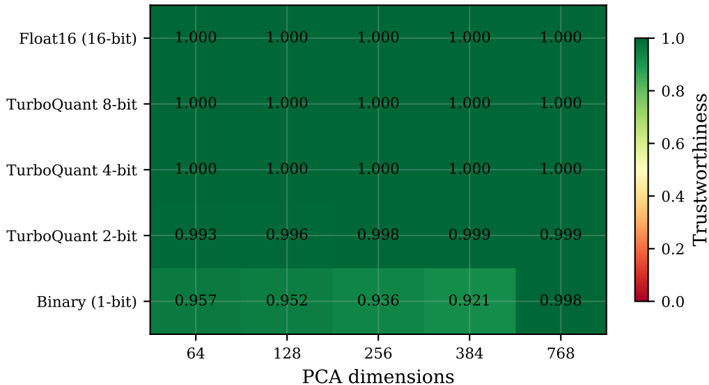
scifact — Trustworthiness (k=10)
