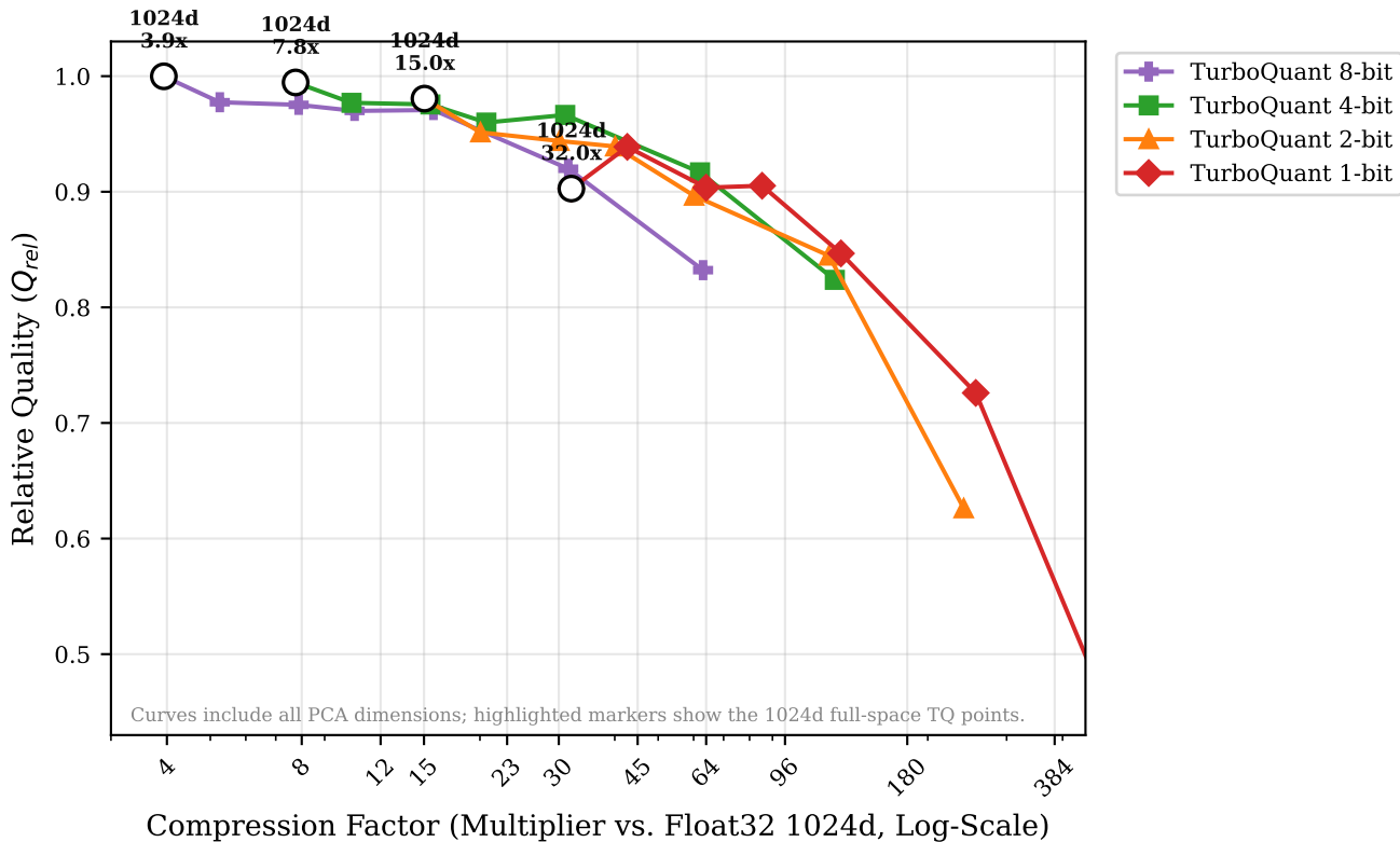
Quality vs. Compression Factor (TurboQuant, 1024d Highlighted)
