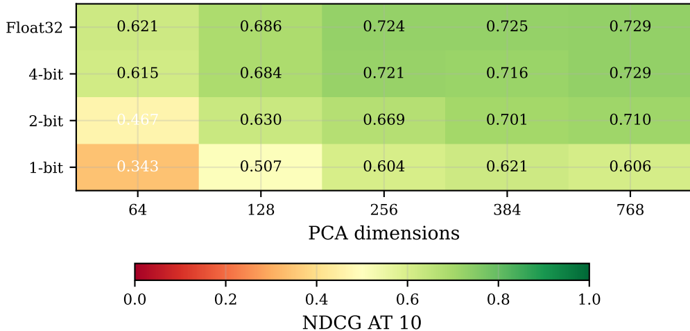
scifact - NDCG@10
