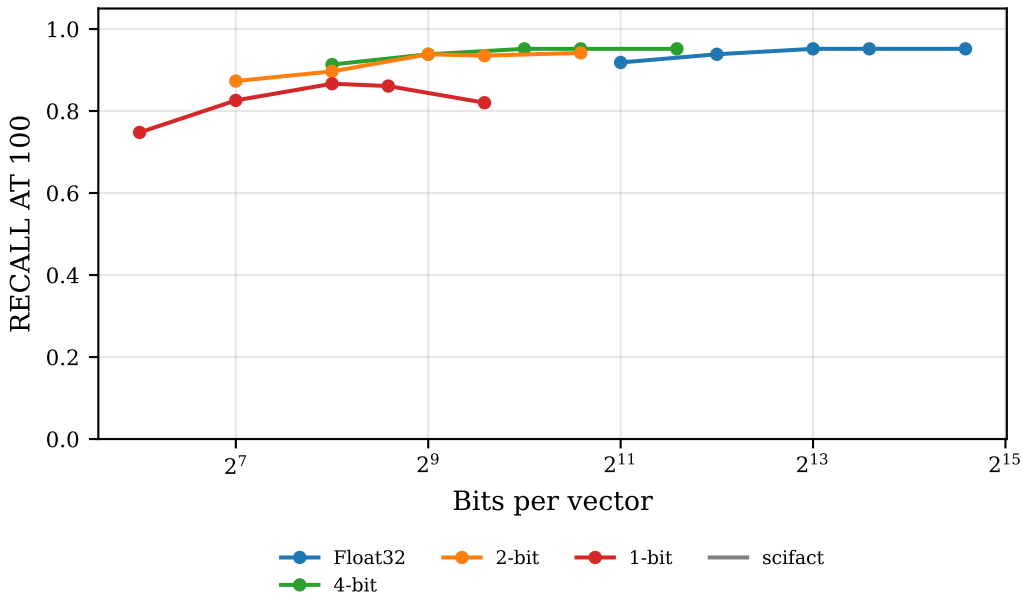
Retrieval RECALL AT 100 vs. Compression
